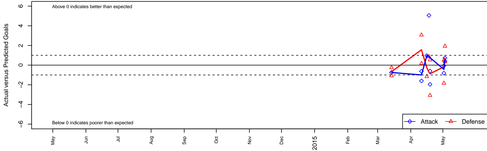
PVSC United B98 Dots are actual minus expected GF (blue circles) and GA (red triangles). Blue line is smoothed change in attack strength. Red is smoothed change in defense strength.
